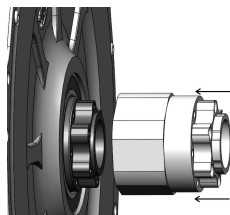
Figure 4: Axle Extender.
