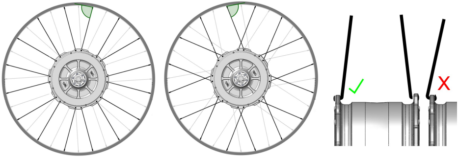
Figure 12: 0 Cross (left) works OK, but for 24" and larger 1 cross (middle) is recommended. Even if dishing optimization suggests otherwise, lace both left and right side spokes with elbows in.
