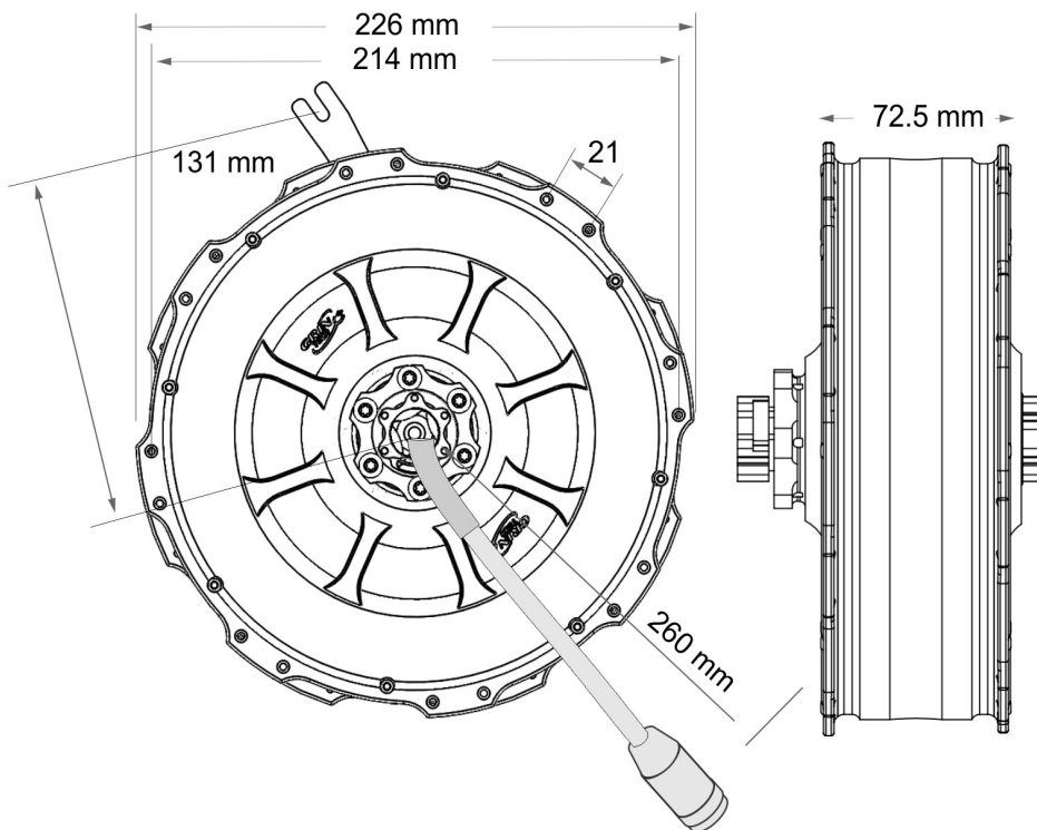
Figure 15: Mechanical Drawing. Detailed drawings with various adapters are available in a separate document.
