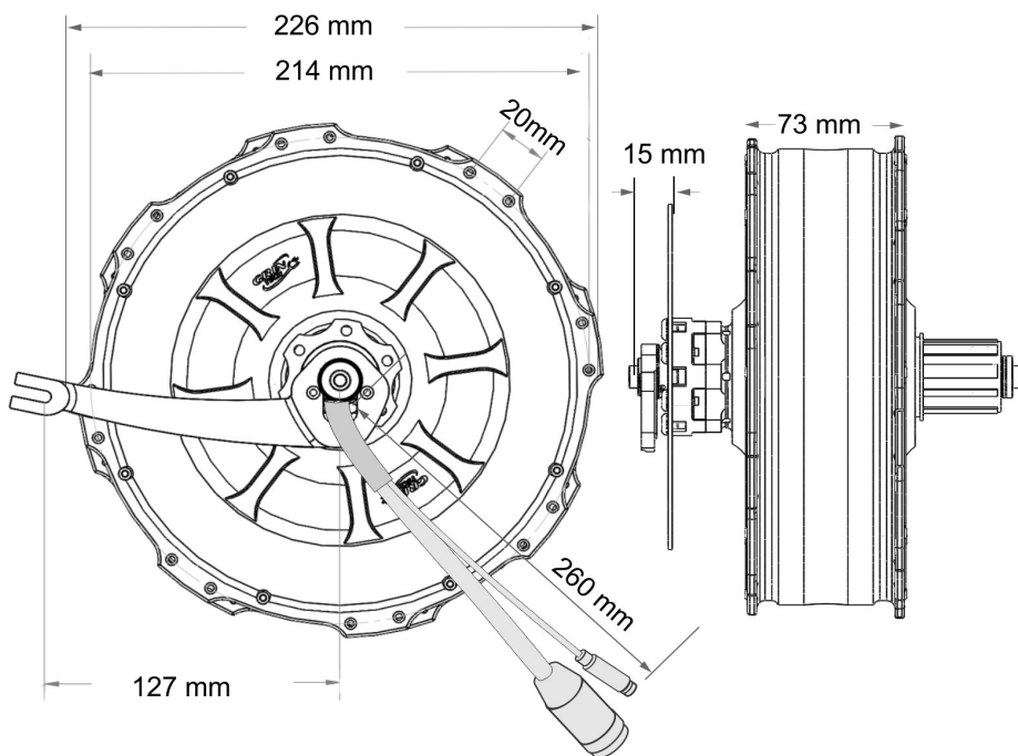
Figure 22: Mechanical Drawing. Fully detailed drawings with all the various axle adapters are available as separate .pdf downloads
