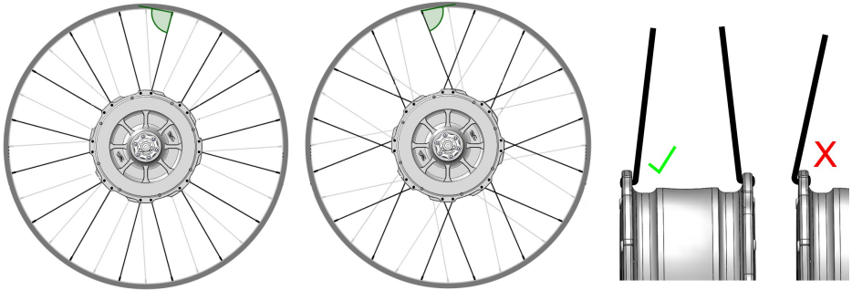
Figure 18: 0 Cross (left) works, but for 24" and larger 1 cross (middle) is recommended. Even if dishing optimization suggests otherwise, lace both left and right side spokes with elbows in.
